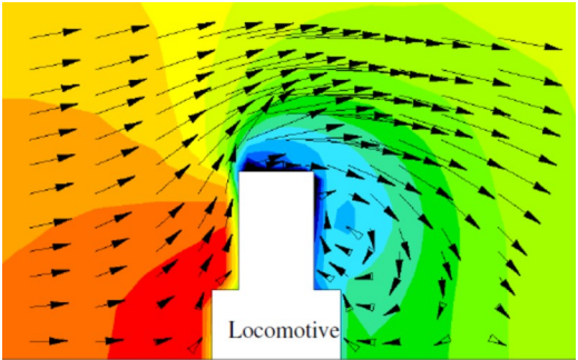
Figure 2: Recirculation Patterns Can Occur Because of Wind and Train Motion
